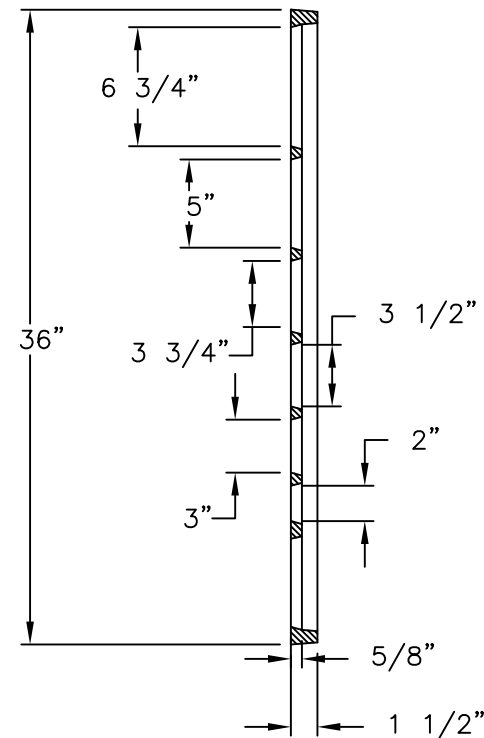
HALF GRATE SECTION
