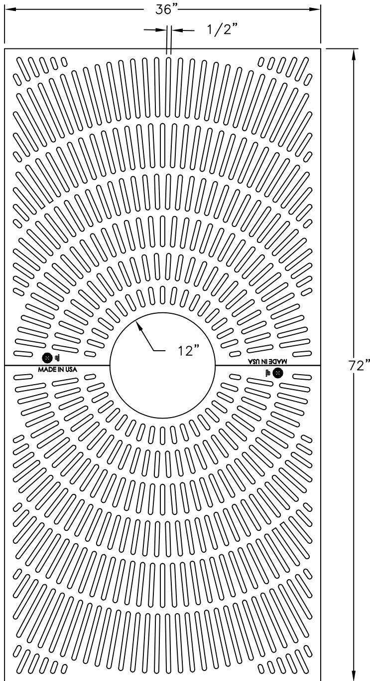
PLAN VIEW
